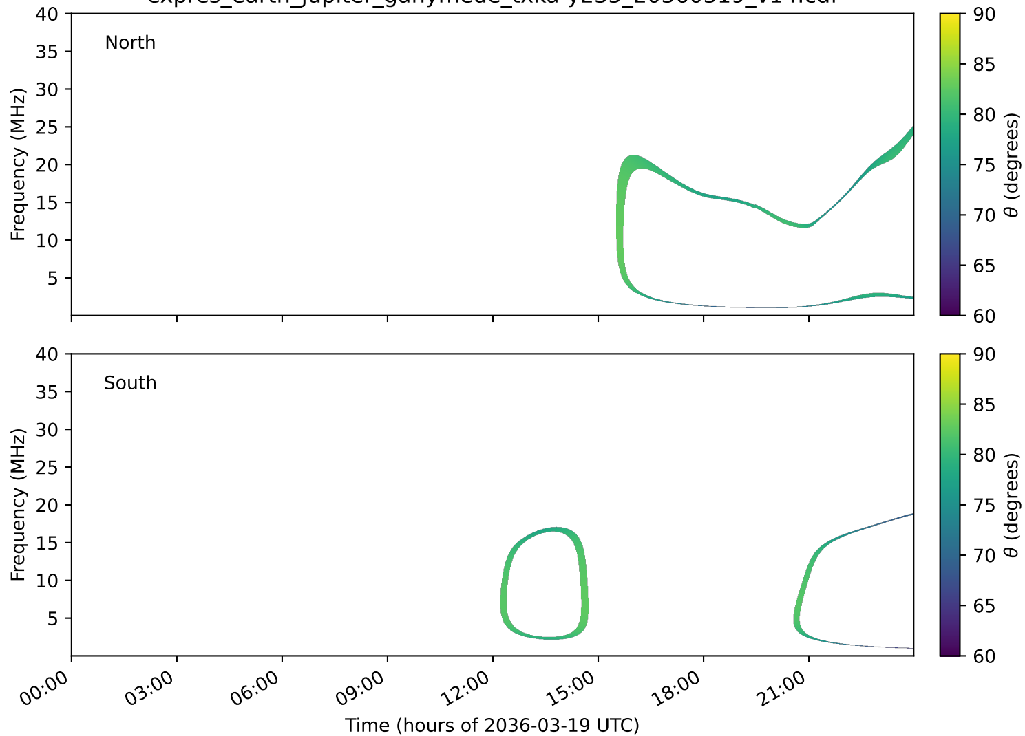
expres_earth_jupiter_ganymede_txka-y235_20360319_v14.cdf
