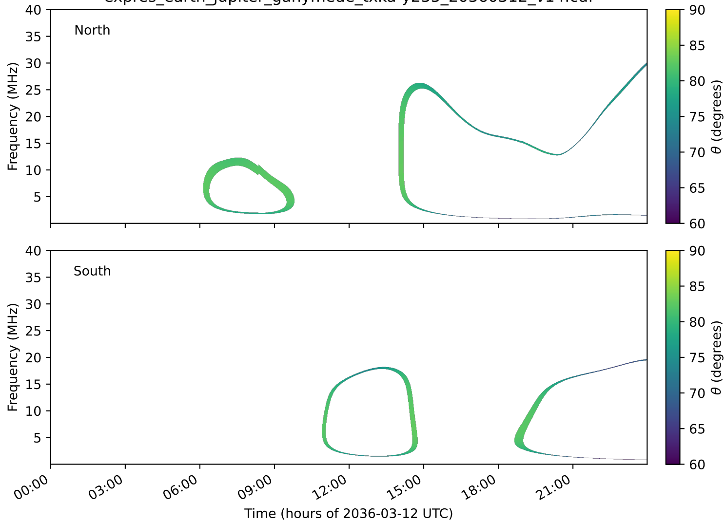
expres_earth_jupiter_ganymede_txka-y235_20360312_v14.cdf
