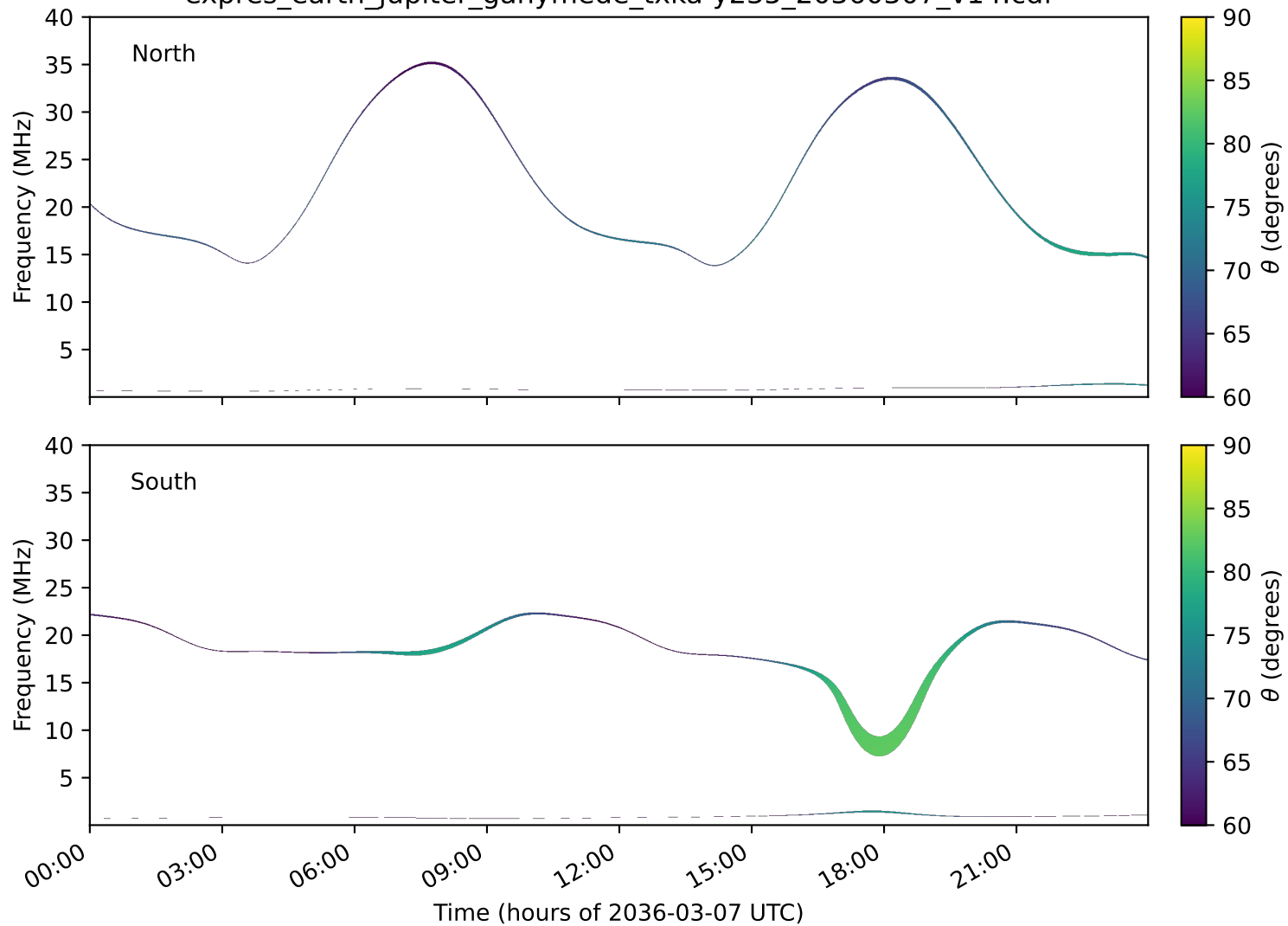
expres_earth_jupiter_ganymede_txka-y235_20360307_v14.cdf
