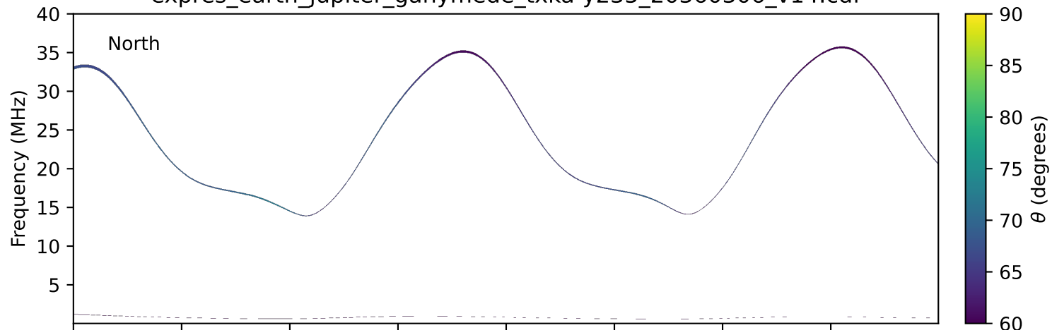
expres_earth_jupiter_ganymede_txka-y235_20360306_v14.cdf
