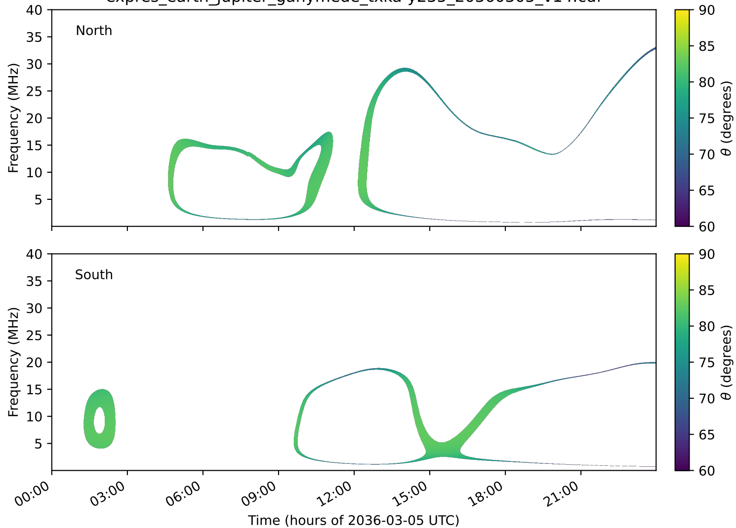
expres_earth_jupiter_ganymede_txka-y235_20360305_v14.cdf
