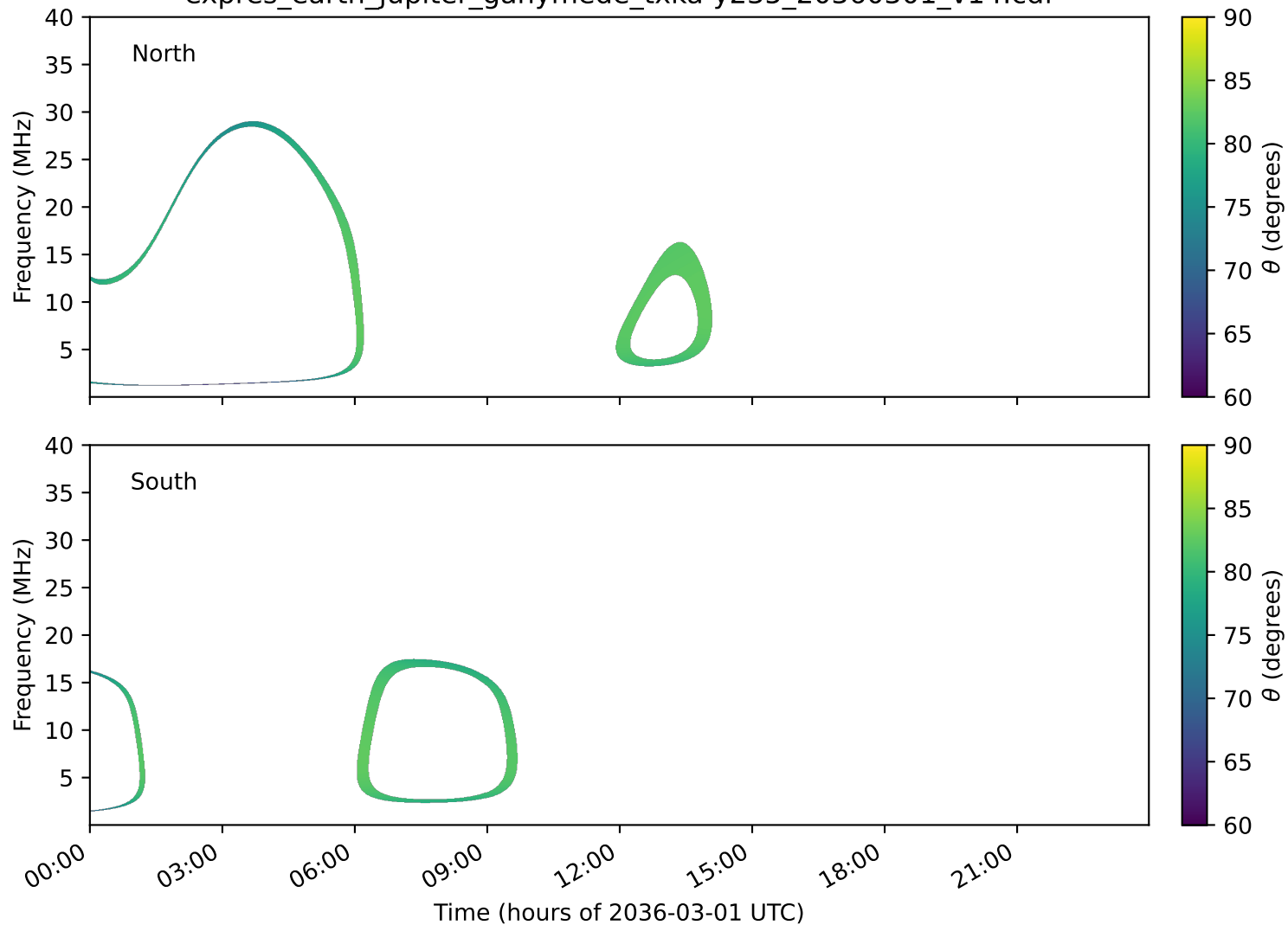
expres_earth_jupiter_ganymede_txka-y235_20360301_v14.cdf
