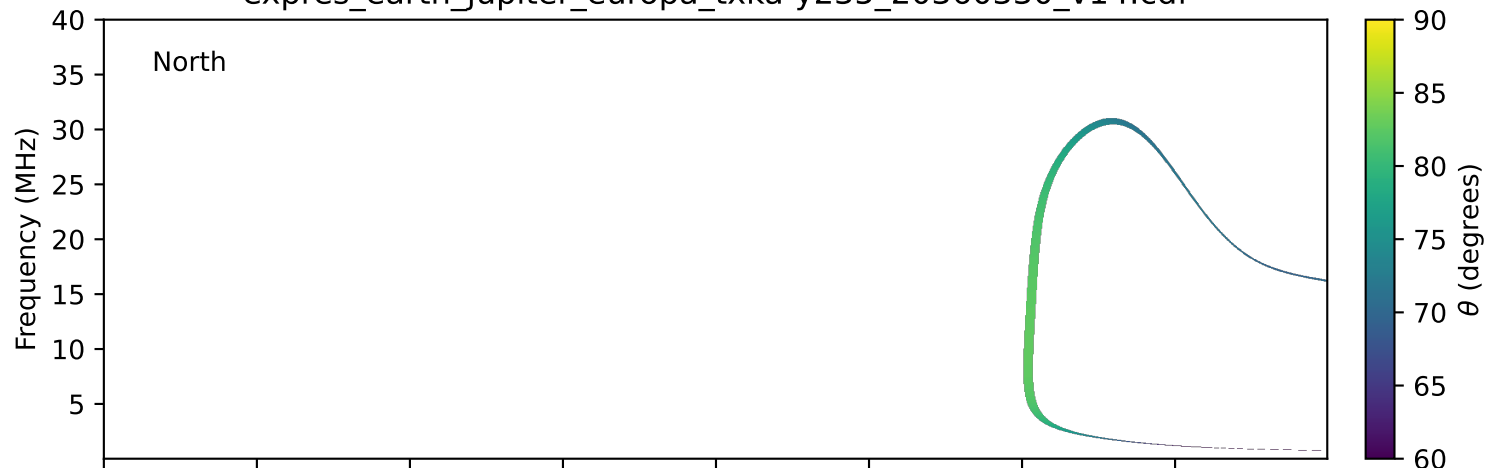
expres_earth_jupiter_europa_txka-y235_20360330_v14.cdf
