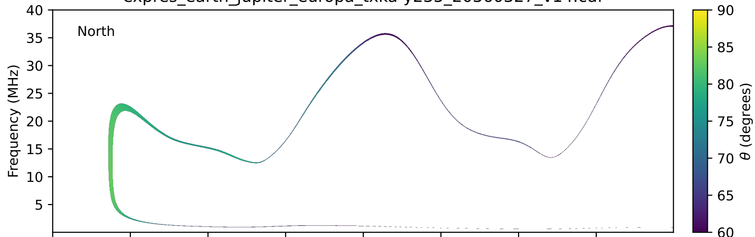
expres_earth_jupiter_europa_txka-y235_20360327_v14.cdf
