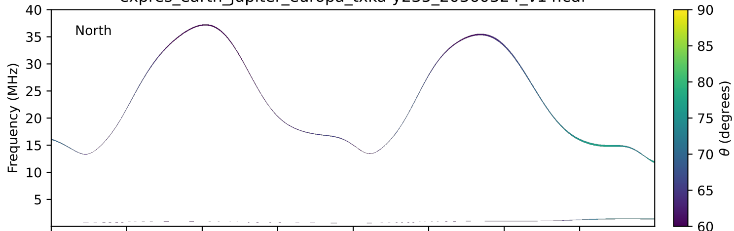
expres_earth_jupiter_europa_txka-y235_20360324_v14.cdf
