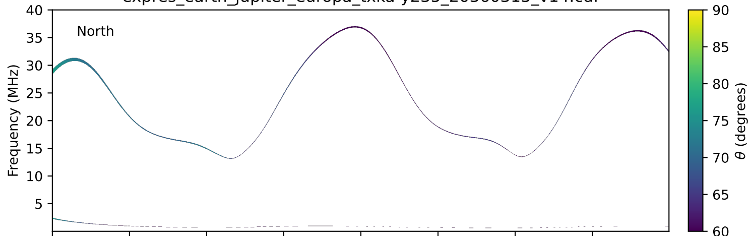
expres_earth_jupiter_europa_txka-y235_20360313_v14.cdf
