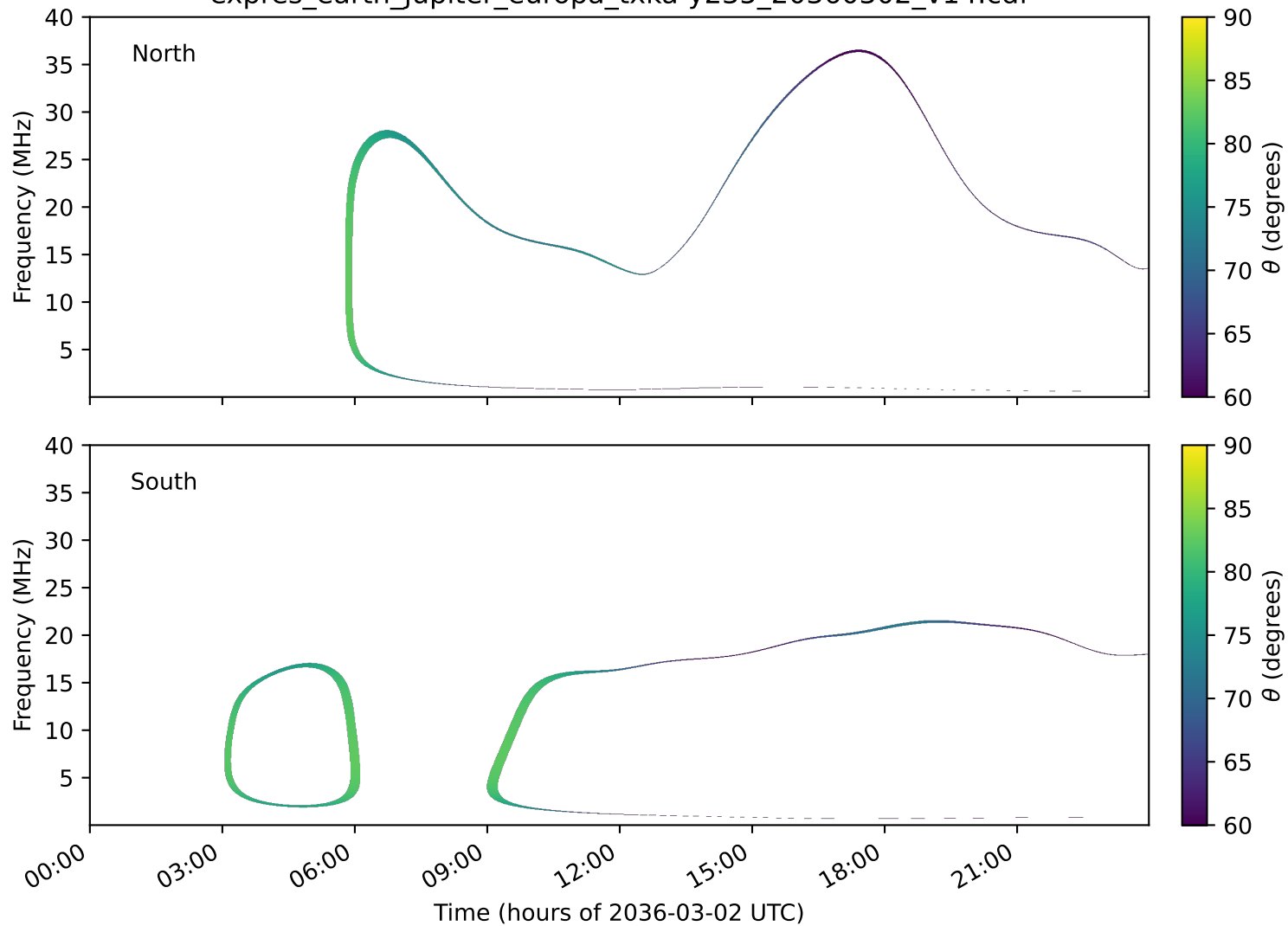
expres_earth_jupiter_europa_txka-y235_20360302_v14.cdf
