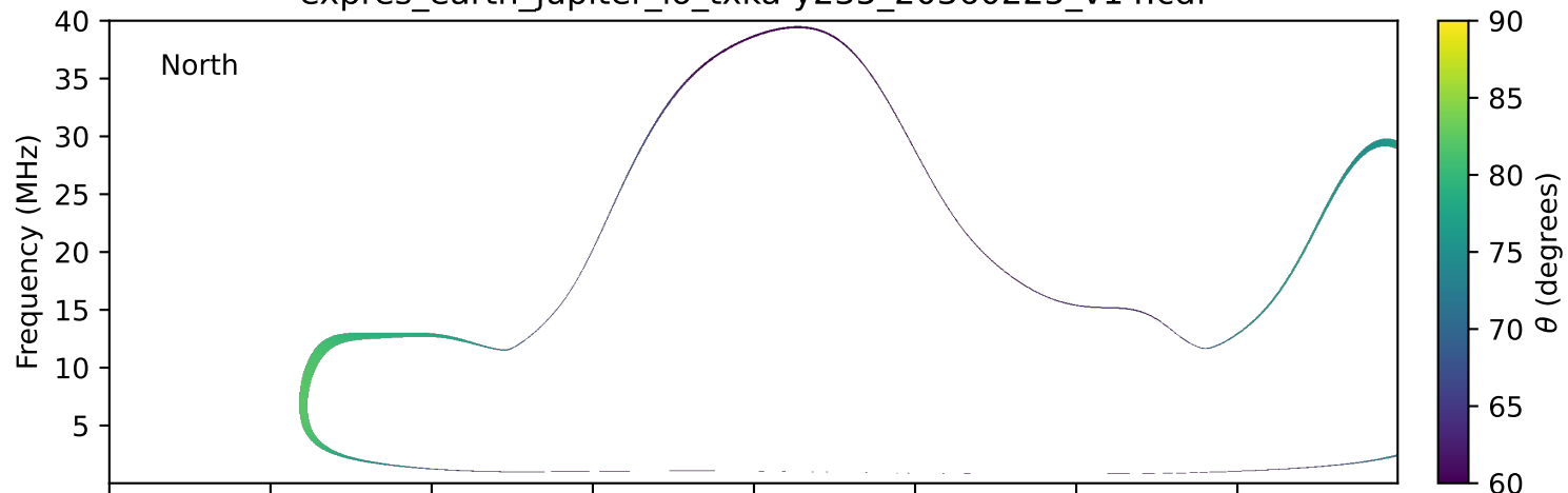
expres_earth_jupiter_io_txka-y235_20360225_v14.cdf
