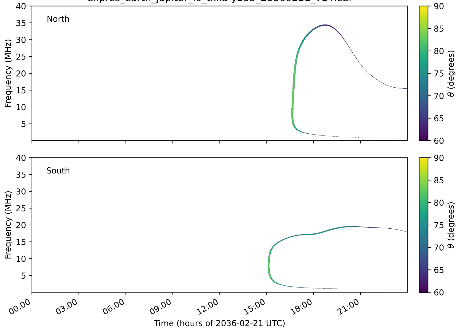
expres_earth_jupiter_io_txka-y235_20360221_v14.cdf
