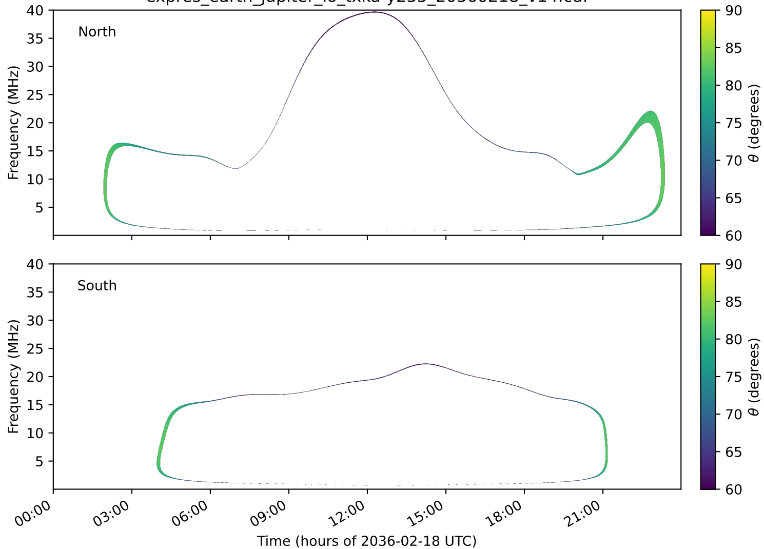
expres_earth_jupiter_io_txka-y235_20360218_v14.cdf
