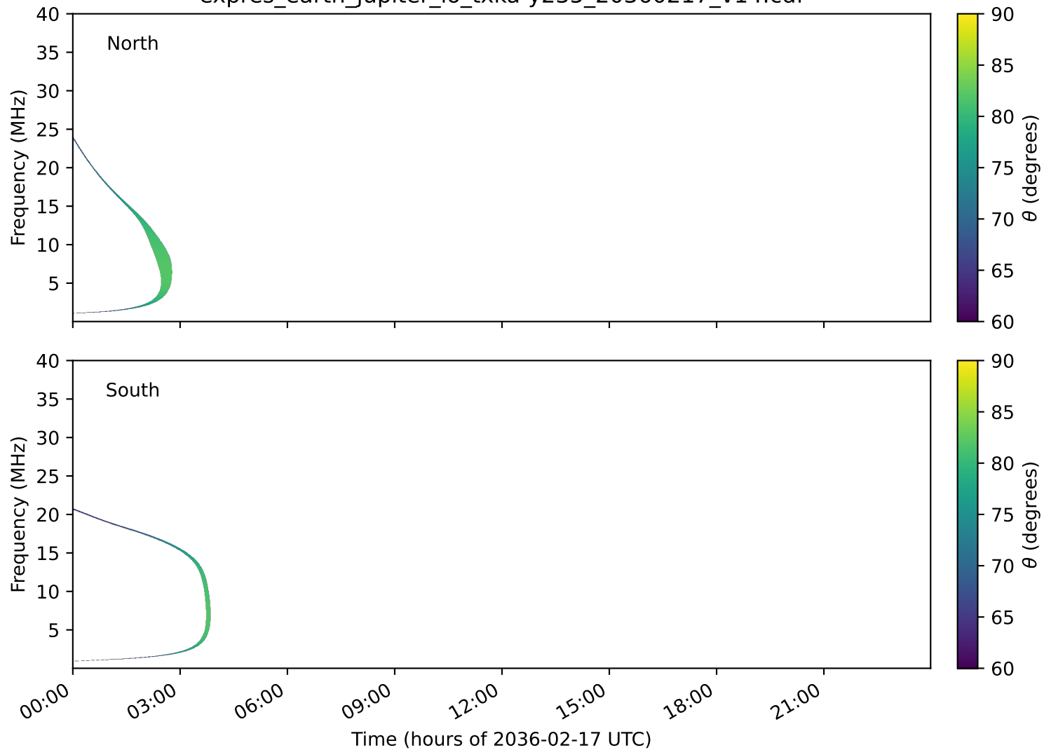
expres_earth_jupiter_io_txka-y235_20360217_v14.cdf
