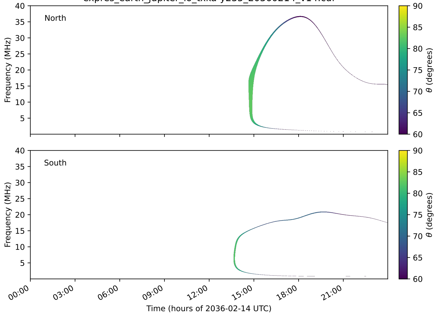
expres_earth_jupiter_io_txka-y235_20360214_v14.cdf
