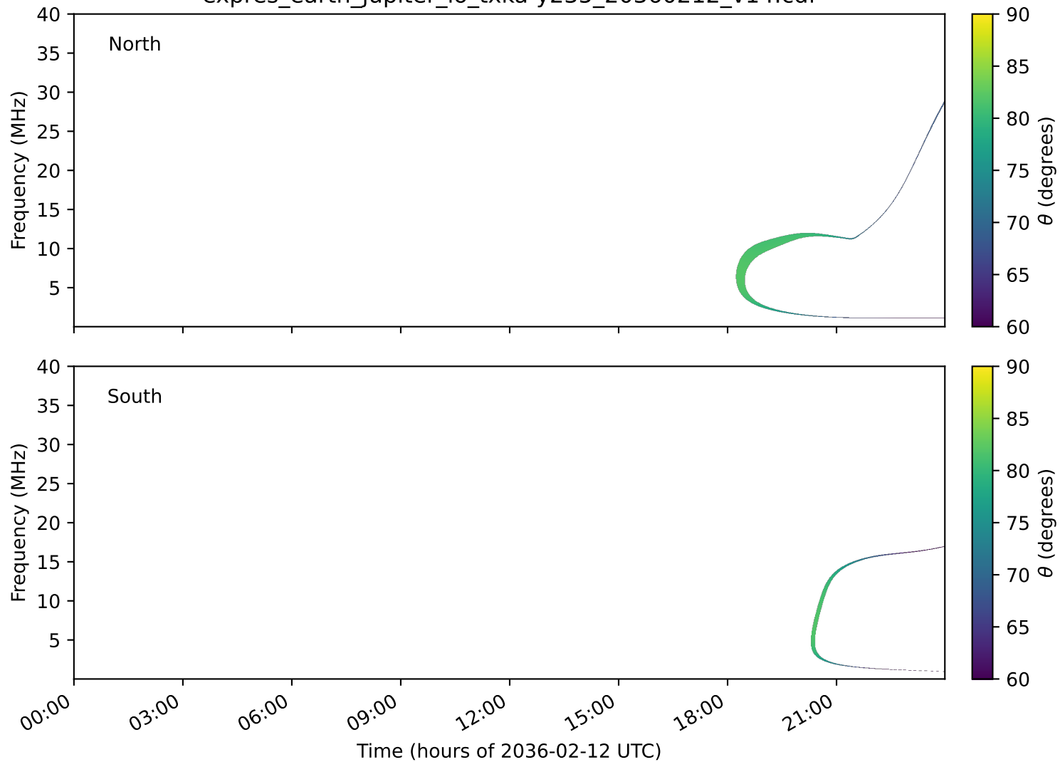
expres_earth_jupiter_io_txka-y235_20360212_v14.cdf
