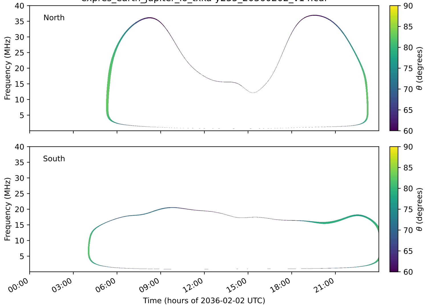
expres_earth_jupiter_io_txka-y235_20360202_v14.cdf
