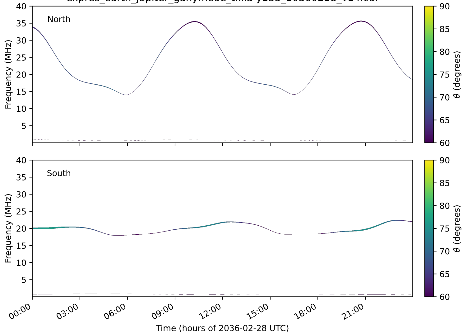
expres_earth_jupiter_ganymede_txka-y235_20360228_v14.cdf
