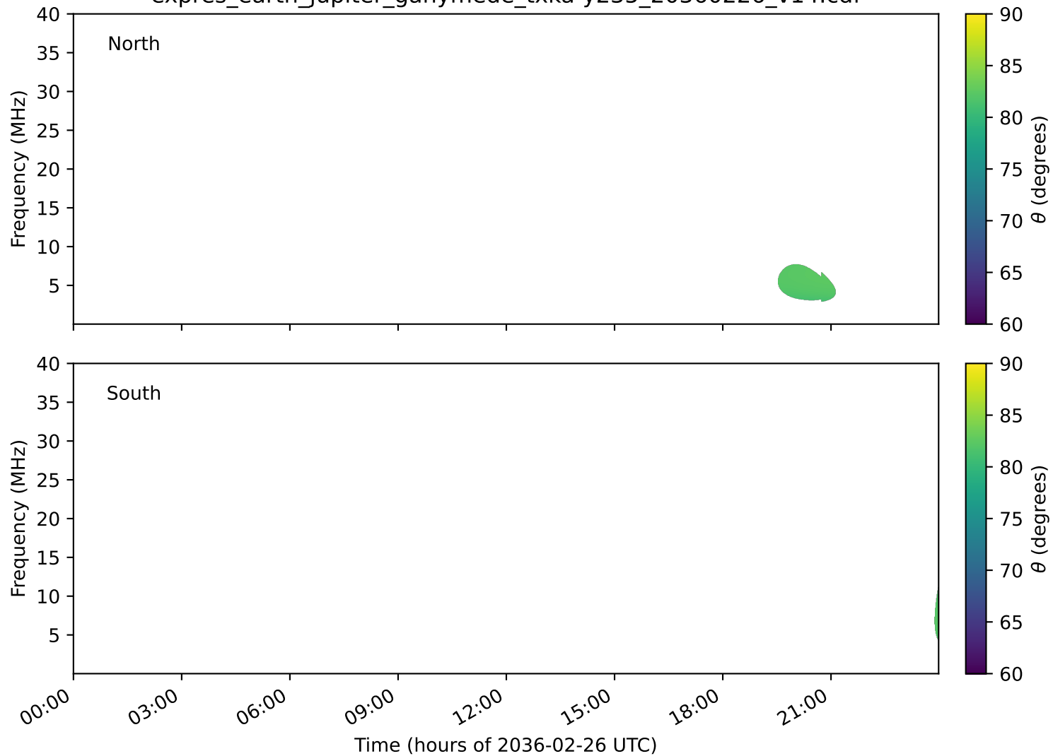
expres_earth_jupiter_ganymede_txka-y235_20360226_v14.cdf
