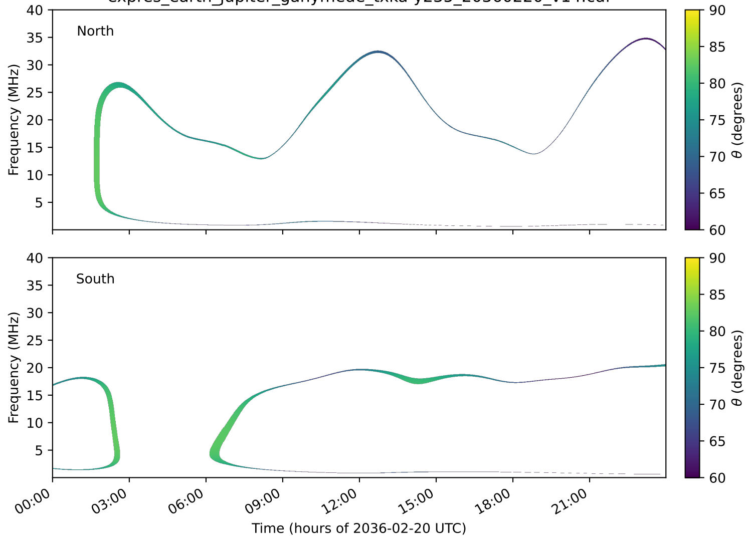
expres_earth_jupiter_ganymede_txka-y235_20360220_v14.cdf
