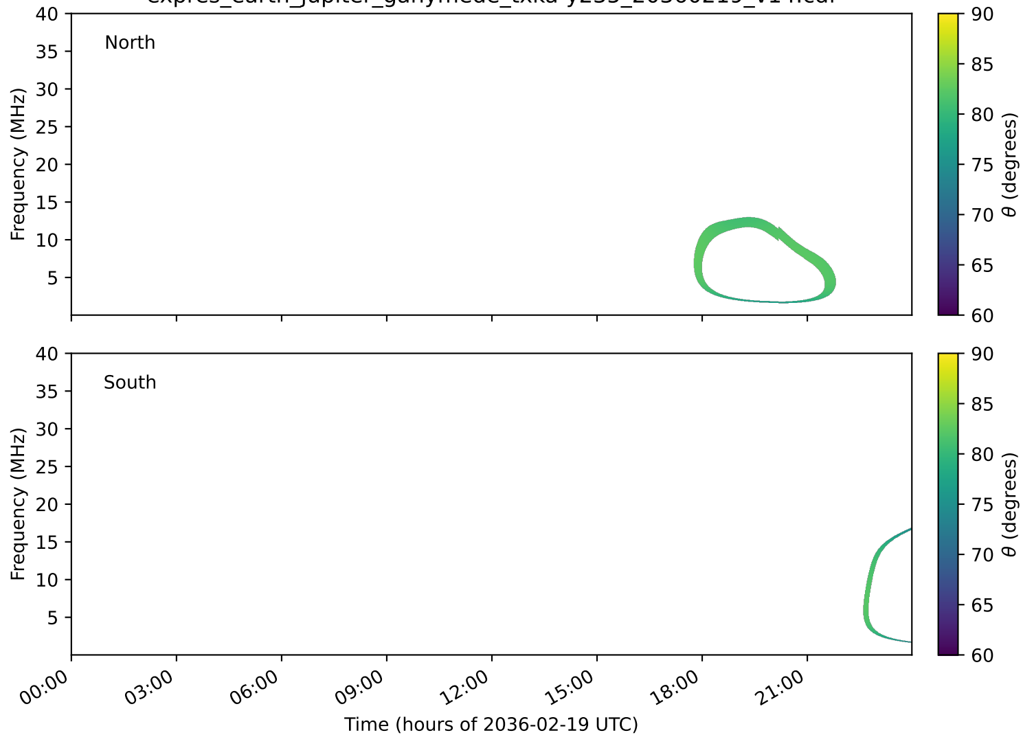
expres_earth_jupiter_ganymede_txka-y235_20360219_v14.cdf
