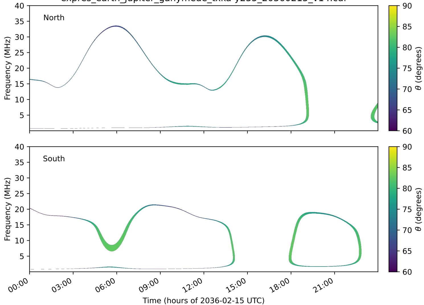
expres_earth_jupiter_ganymede_txka-y235_20360215_v14.cdf
