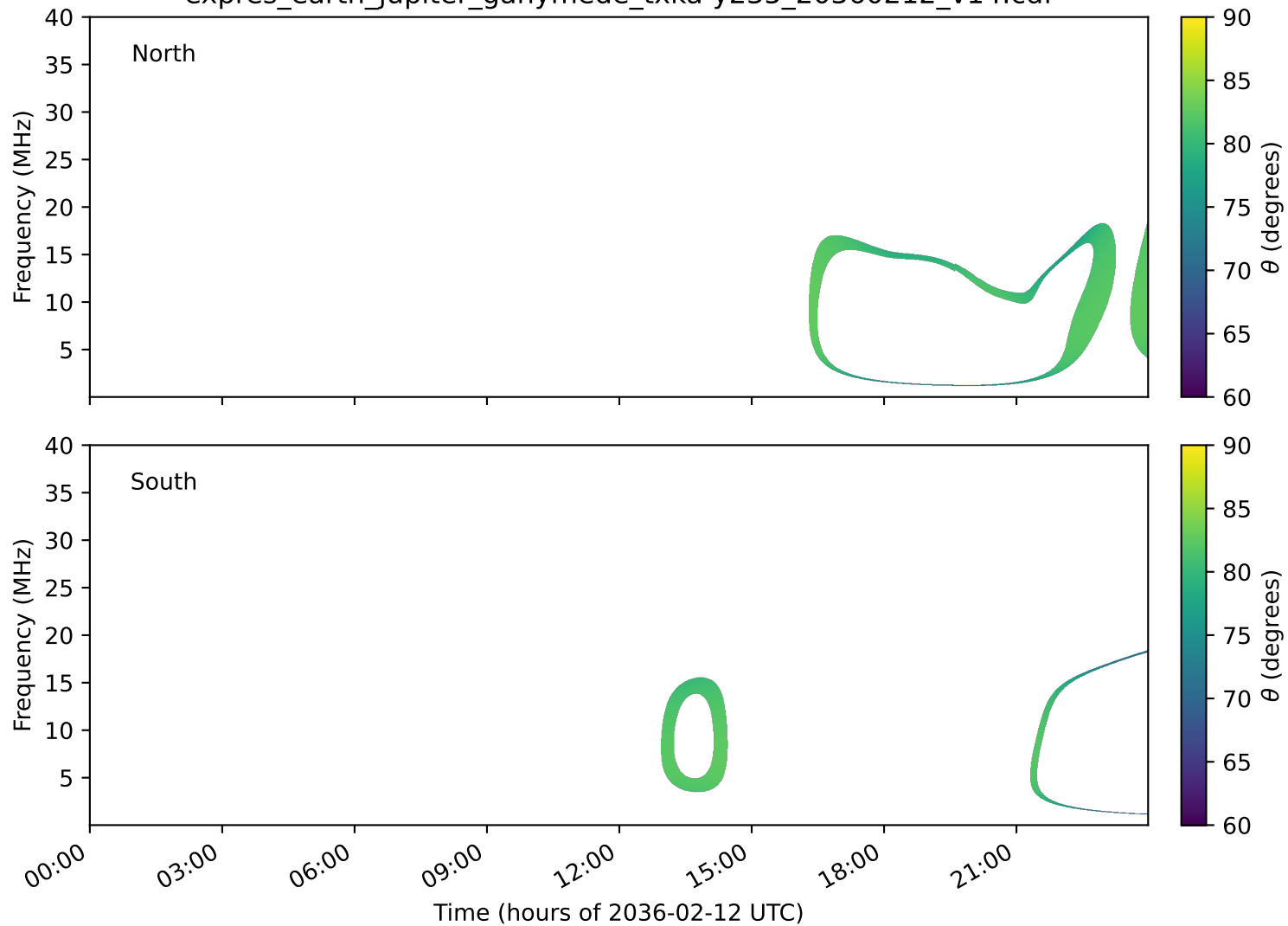
expres_earth_jupiter_ganymede_txka-y235_20360212_v14.cdf
