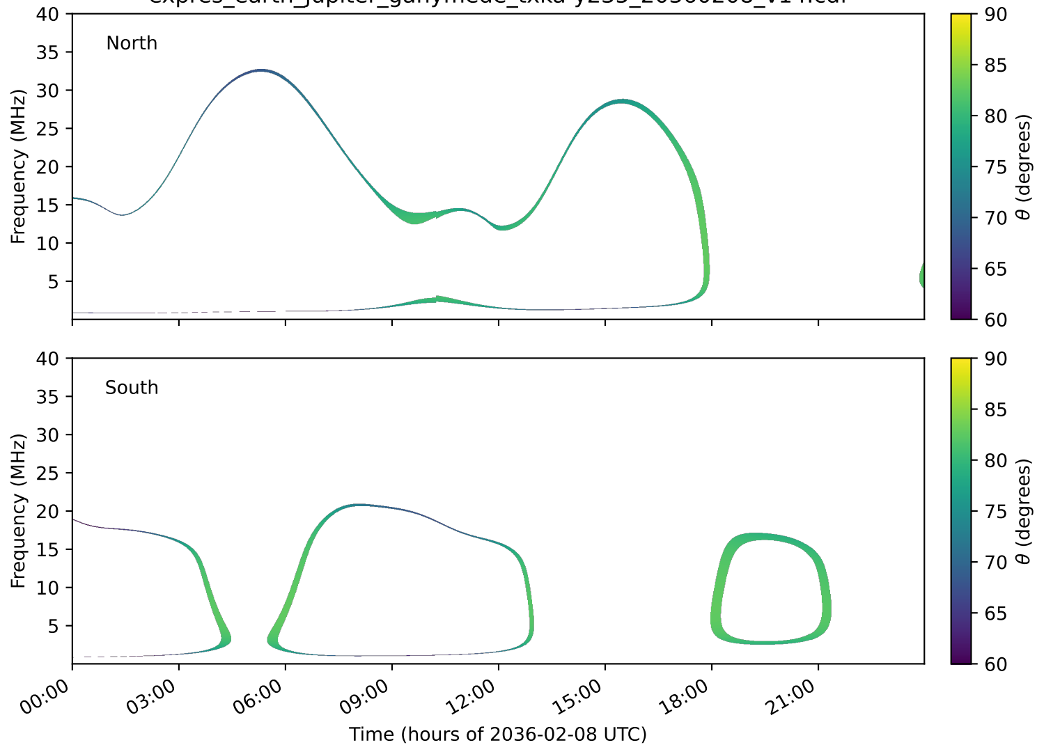
expres_earth_jupiter_ganymede_txka-y235_20360208_v14.cdf
