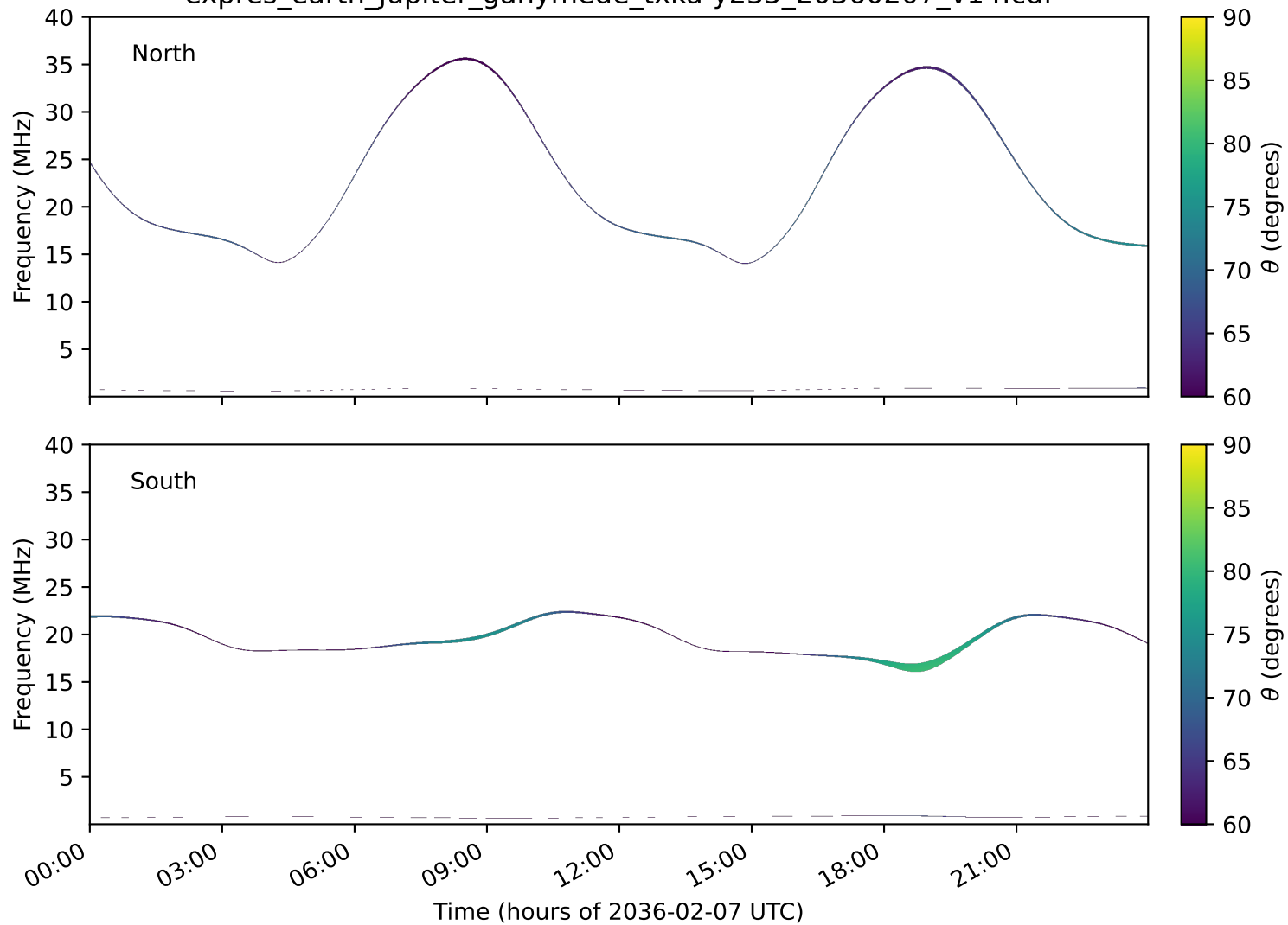
expres_earth_jupiter_ganymede_txka-y235_20360207_v14.cdf
