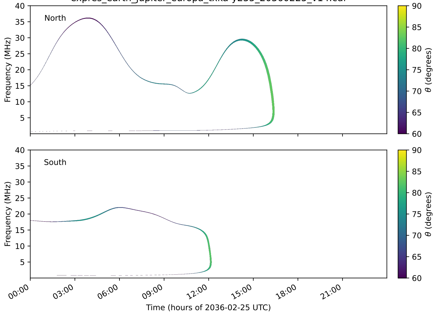
expres_earth_jupiter_europa_txka-y235_20360225_v14.cdf
