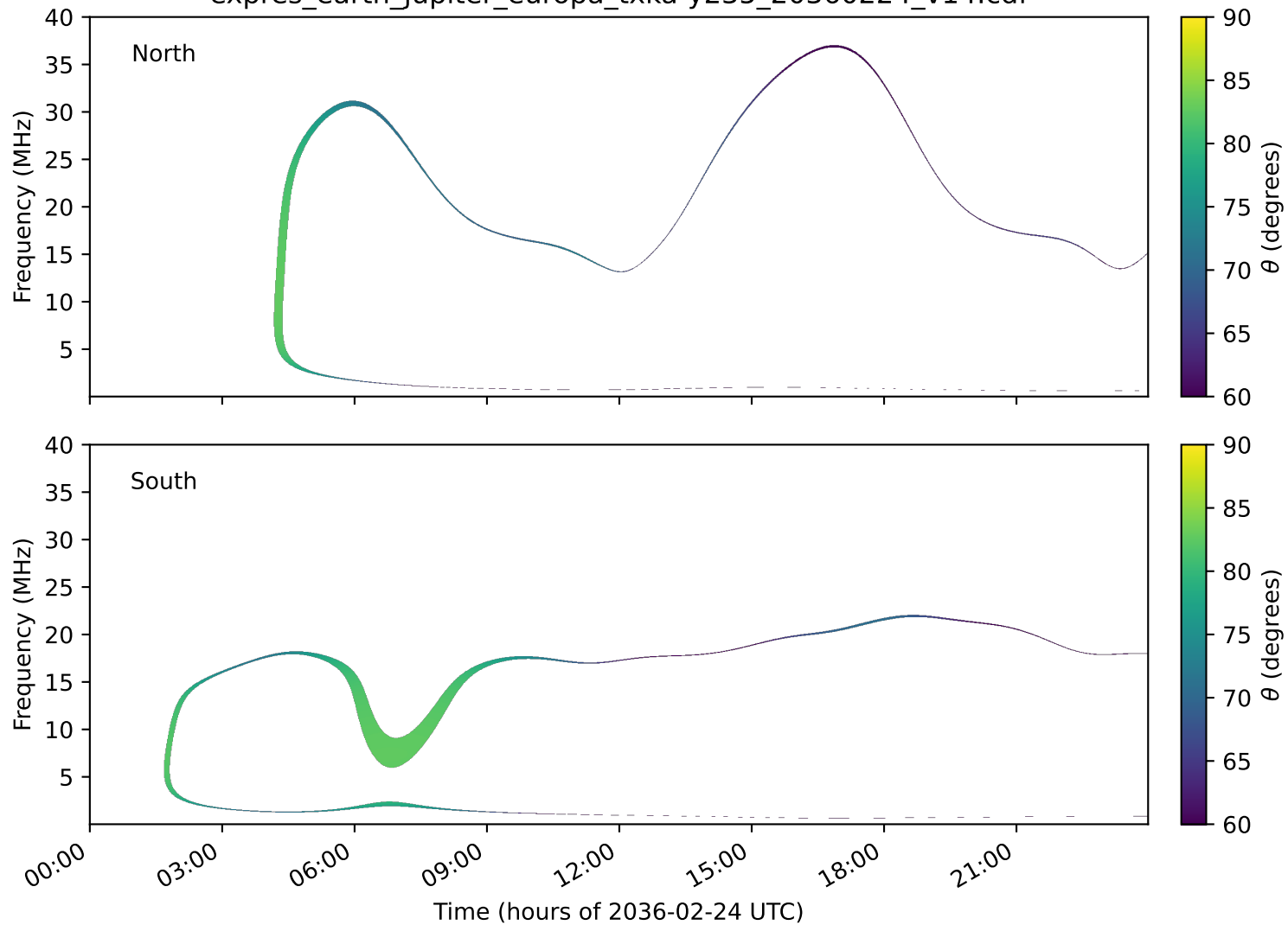
expres_earth_jupiter_europa_txka-y235_20360224_v14.cdf
