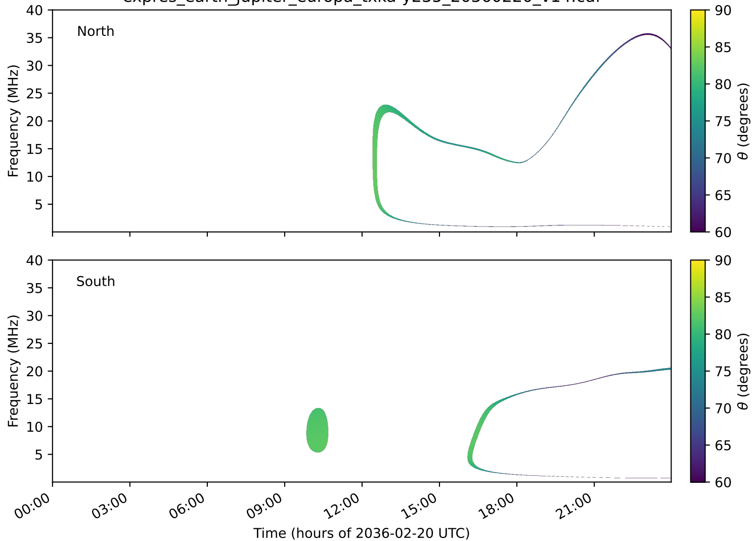
expres_earth_jupiter_europa_txka-y235_20360220_v14.cdf
