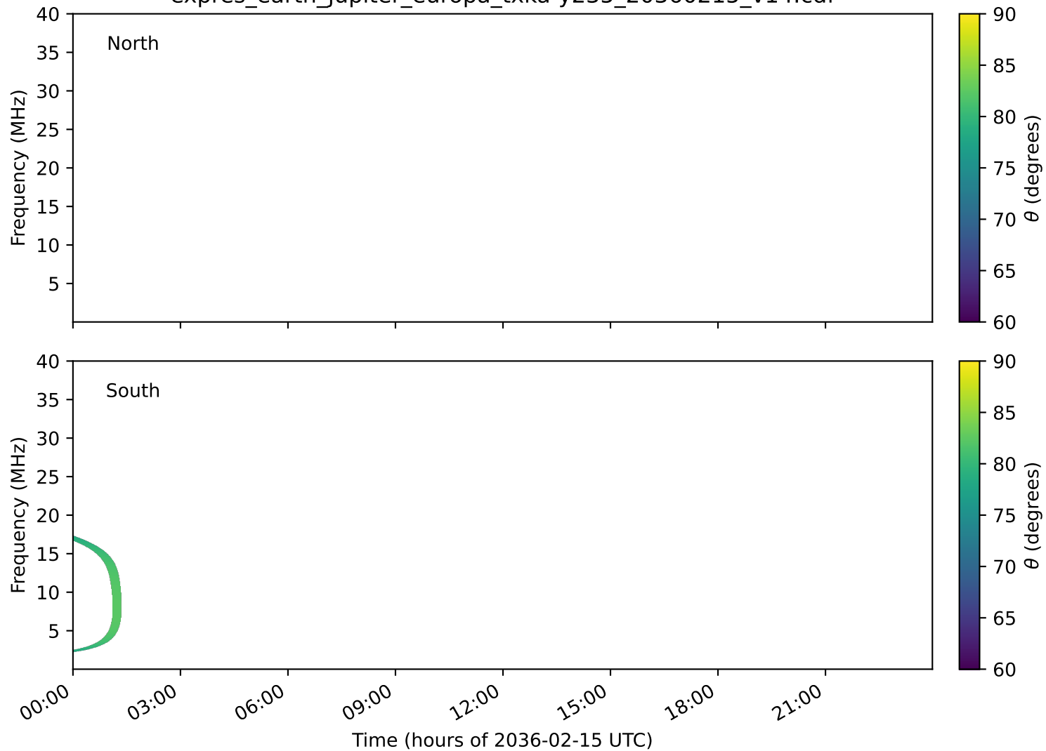
expres_earth_jupiter_europa_txka-y235_20360215_v14.cdf
