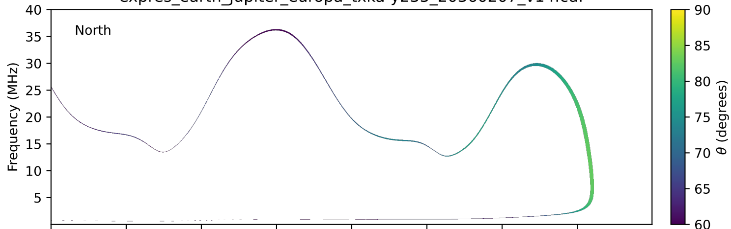
expres_earth_jupiter_europa_txka-y235_20360207_v14.cdf
