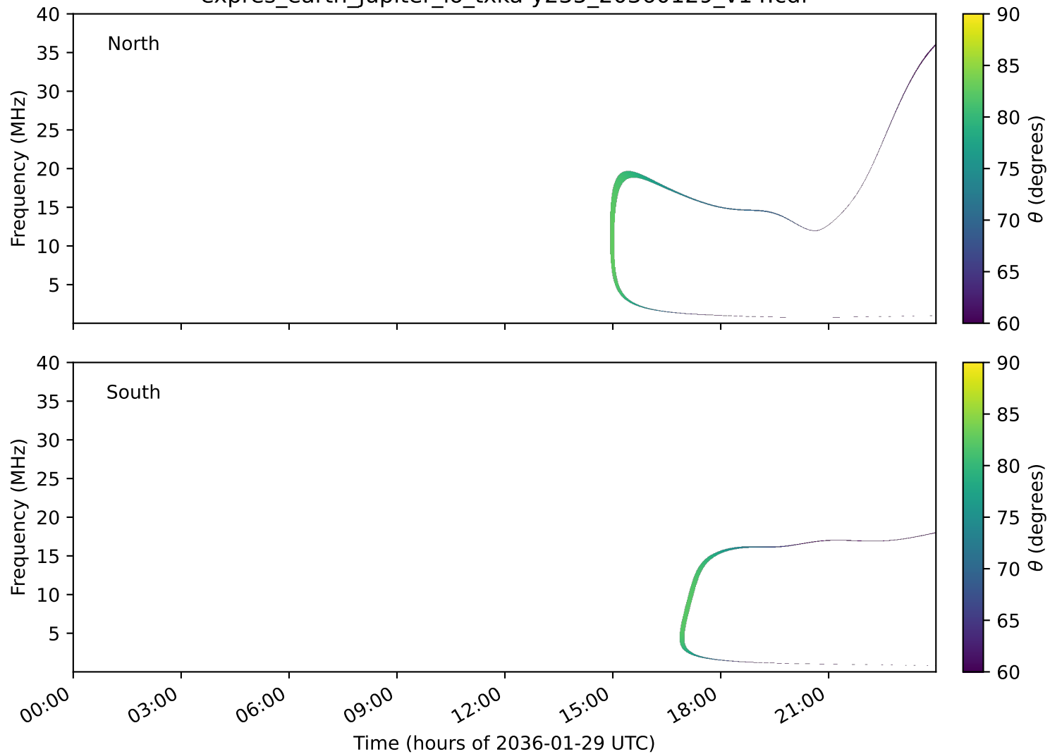
expres_earth_jupiter_io_txka-y235_20360129_v14.cdf
