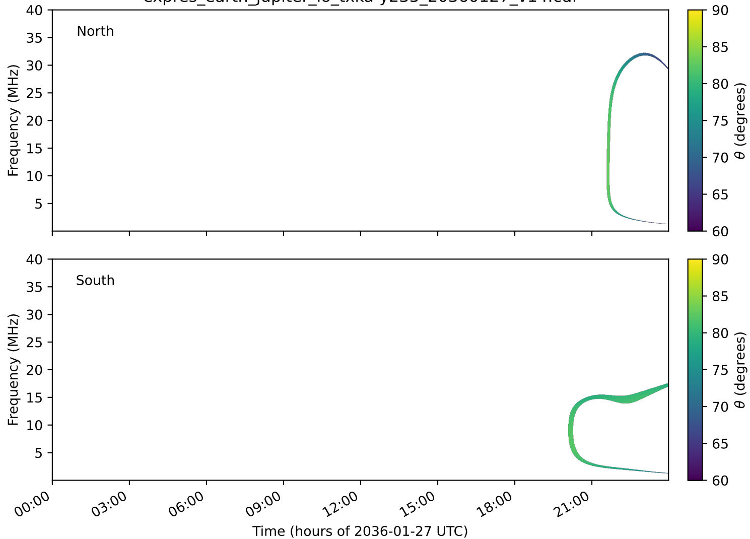
expres_earth_jupiter_io_txka-y235_20360127_v14.cdf
