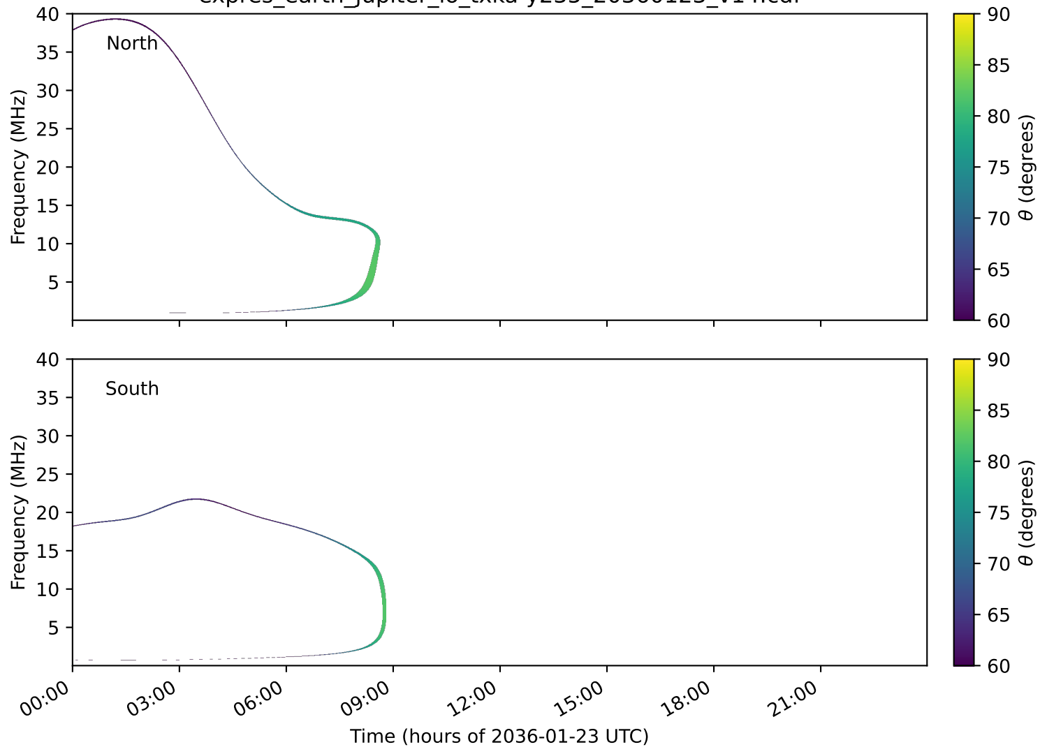
expres_earth_jupiter_io_txka-y235_20360123_v14.cdf
