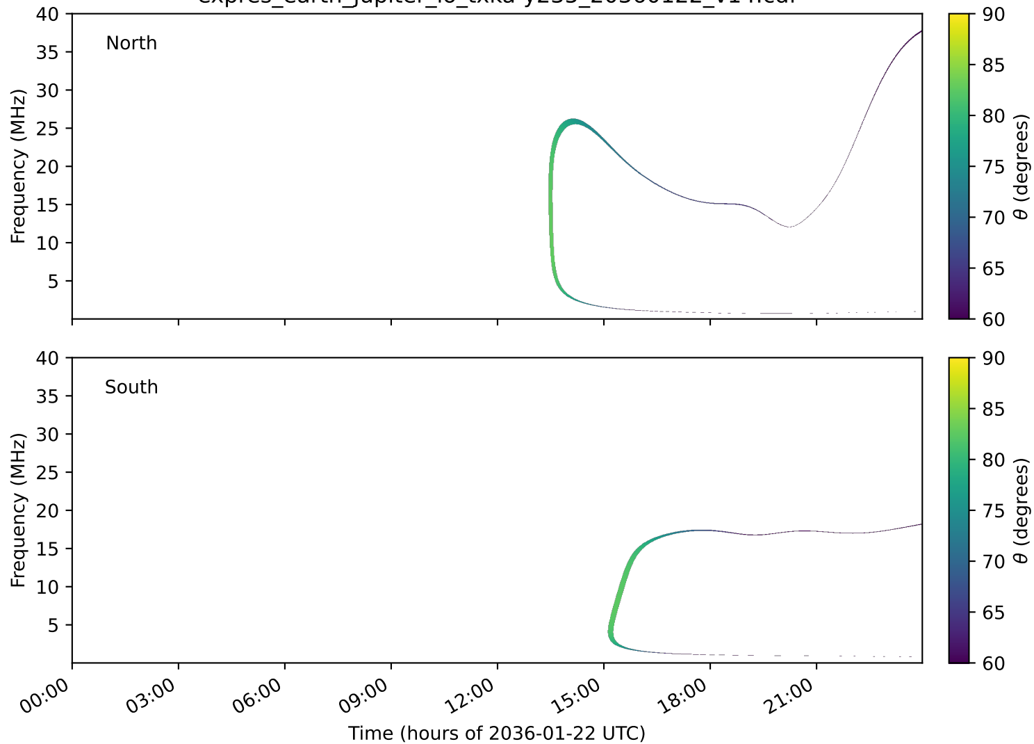
expres_earth_jupiter_io_txka-y235_20360122_v14.cdf
