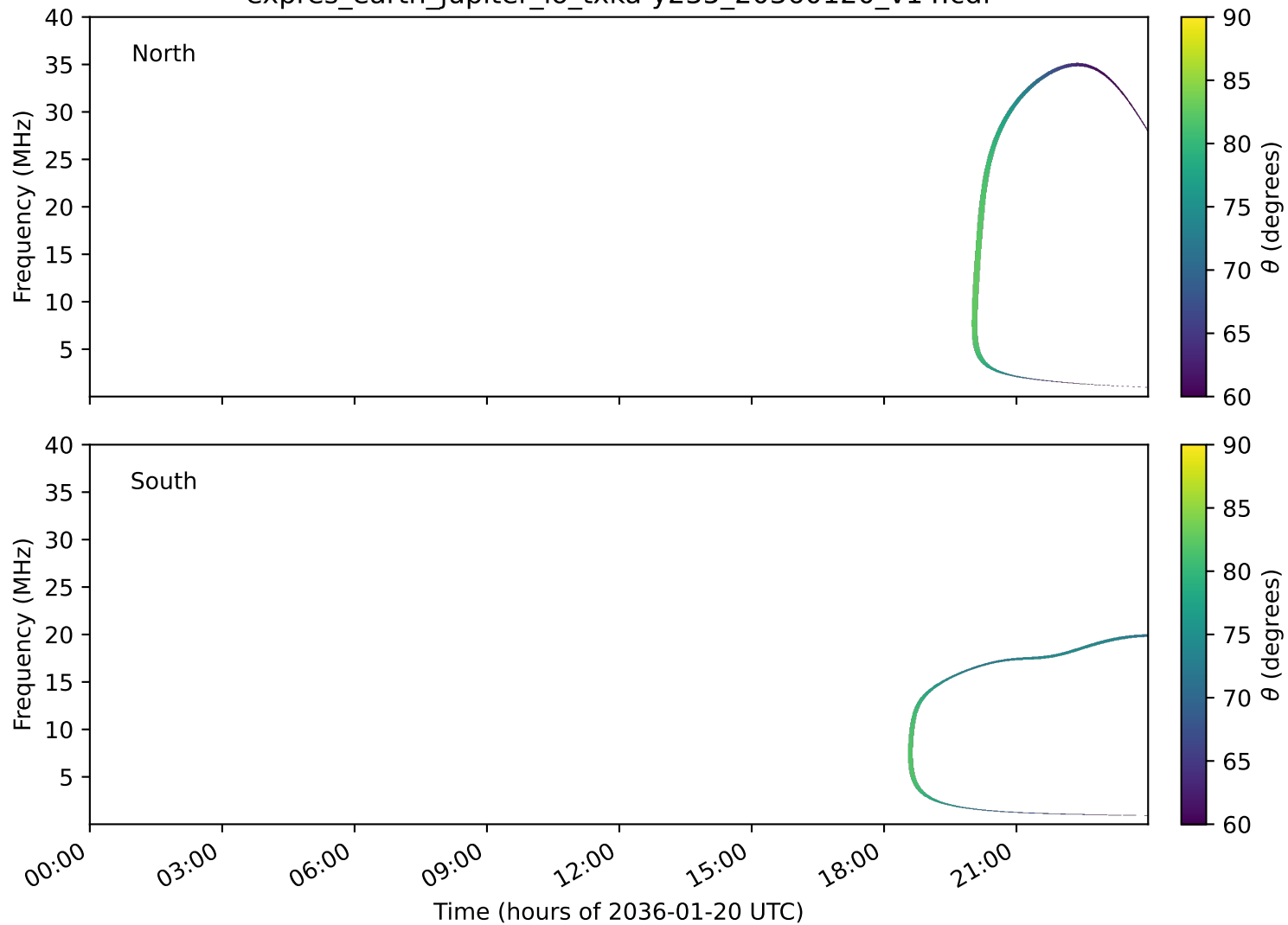
expres_earth_jupiter_io_txka-y235_20360120_v14.cdf
