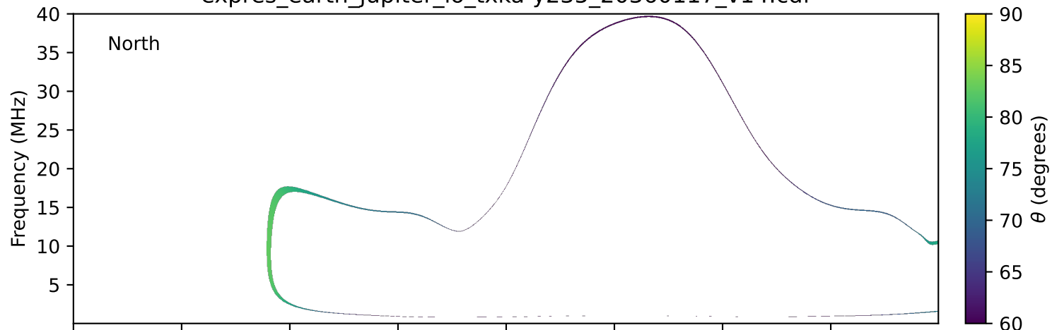
expres_earth_jupiter_io_txka-y235_20360117_v14.cdf
