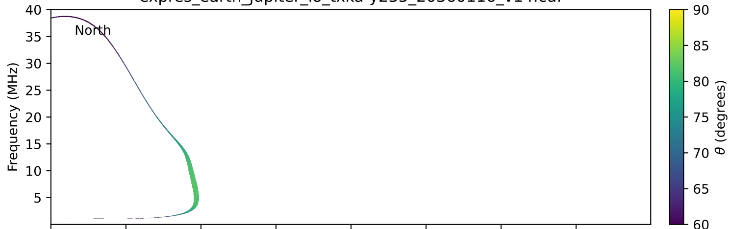
expres_earth_jupiter_io_txka-y235_20360116_v14.cdf
