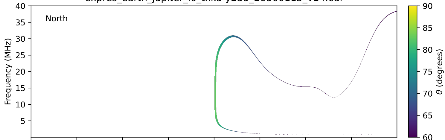
expres_earth_jupiter_io_txka-y235_20360115_v14.cdf
