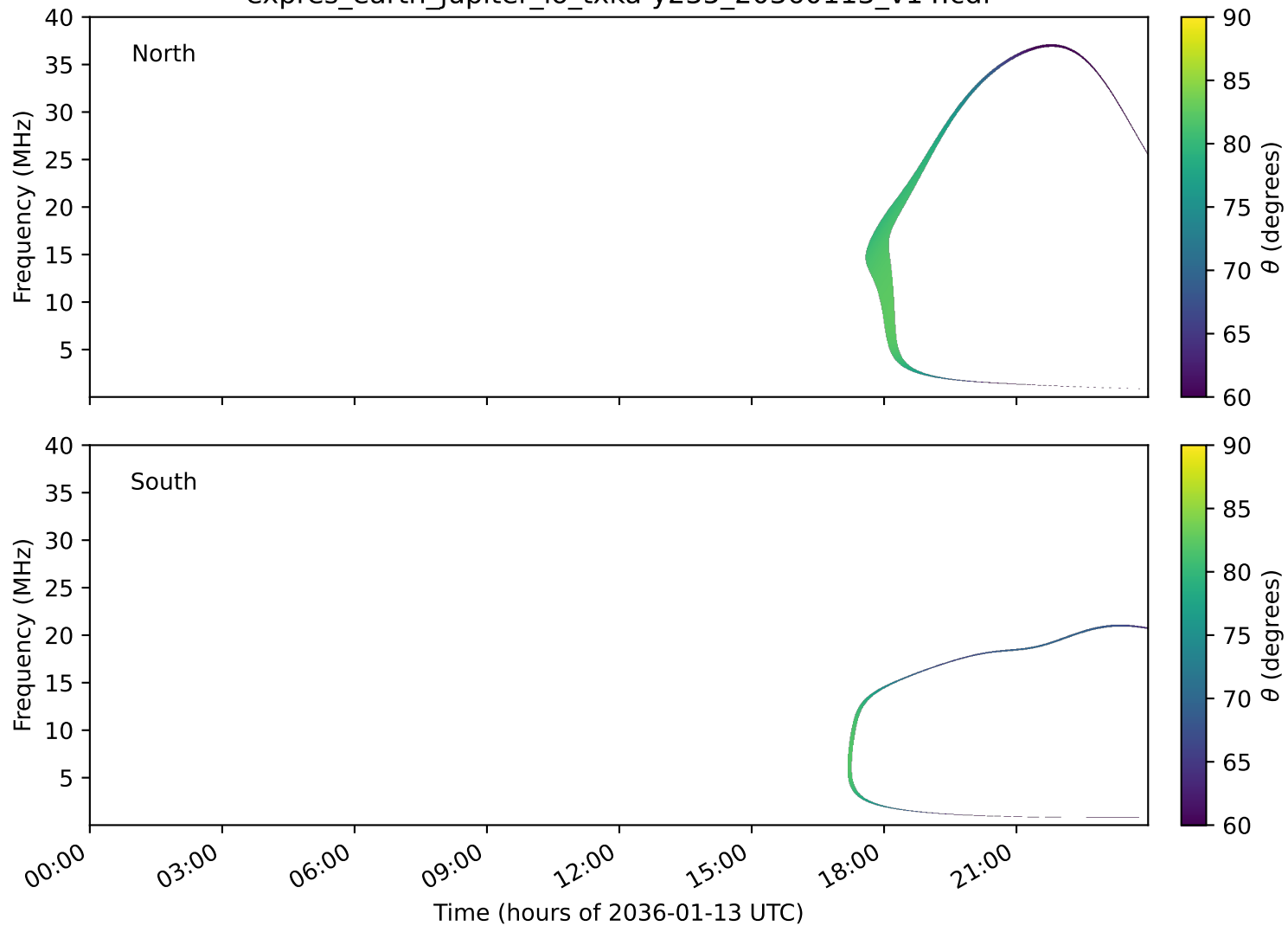
expres_earth_jupiter_io_txka-y235_20360113_v14.cdf
