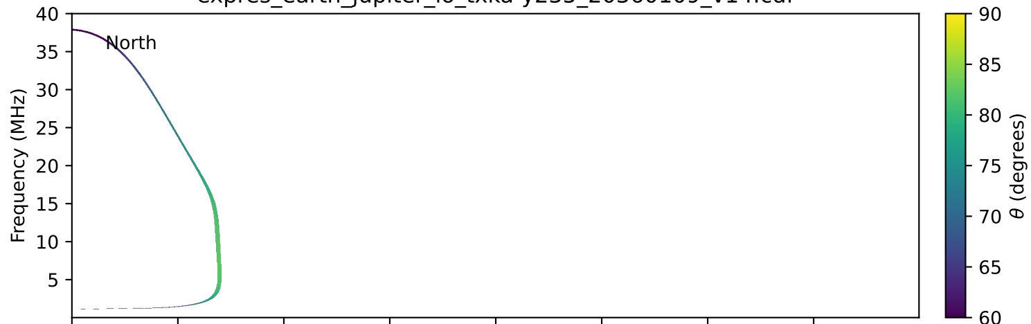
expres_earth_jupiter_io_txka-y235_20360109_v14.cdf
