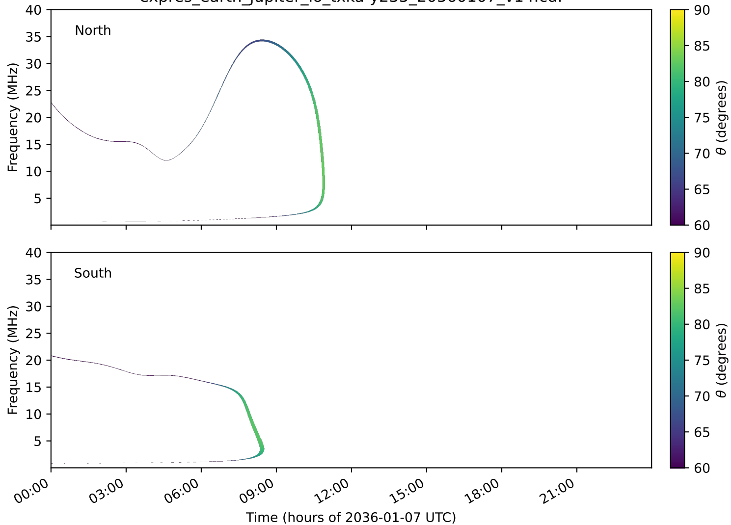
expres_earth_jupiter_io_txka-y235_20360107_v14.cdf
