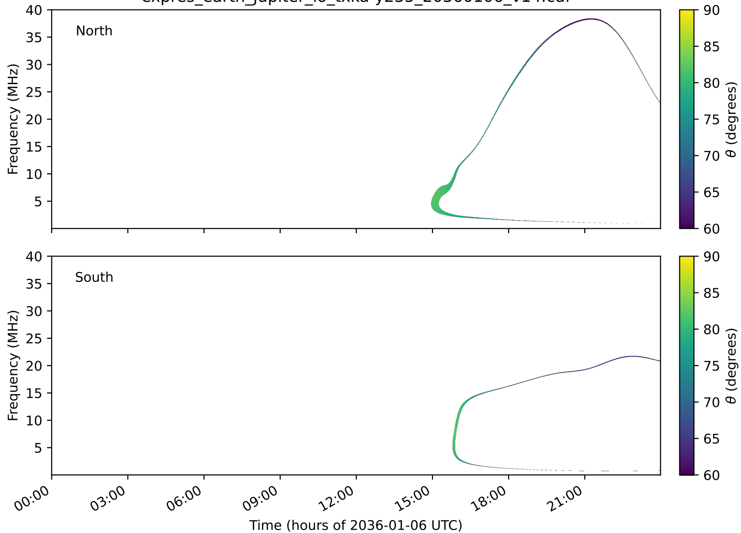
expres_earth_jupiter_io_txka-y235_20360106_v14.cdf
