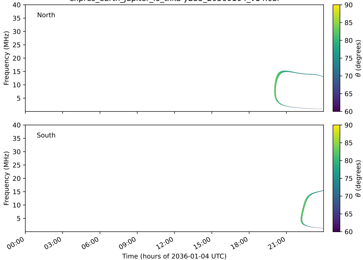
expres_earth_jupiter_io_txka-y235_20360104_v14.cdf
