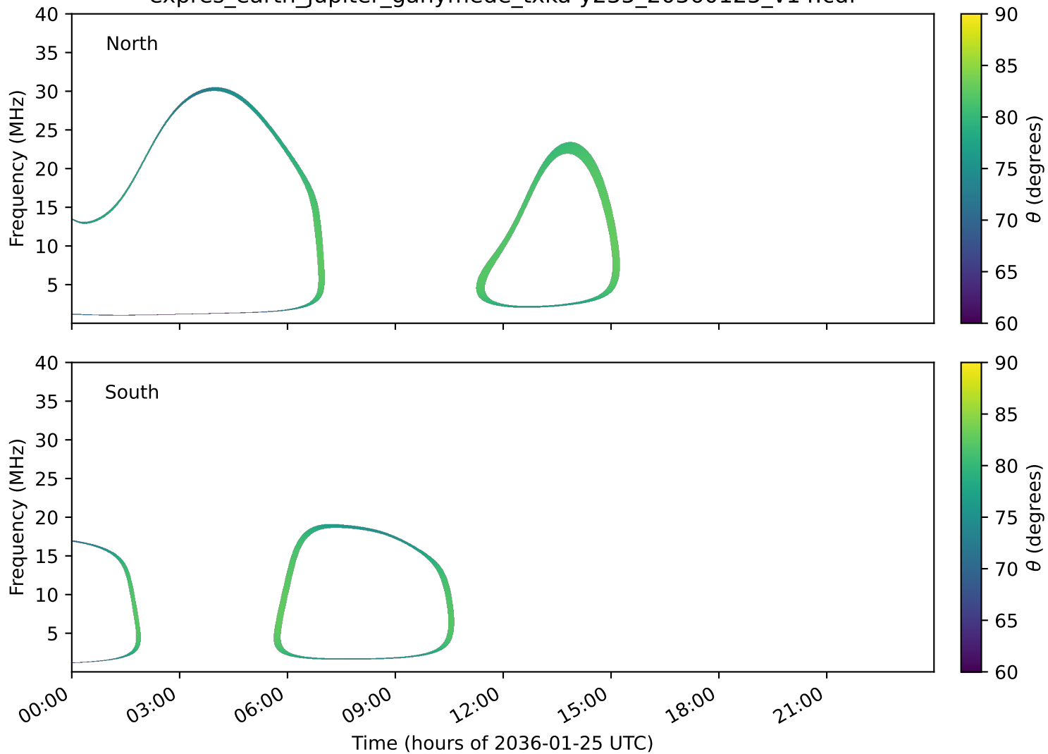
expres_earth_jupiter_ganymede_txka-y235_20360125_v14.cdf
