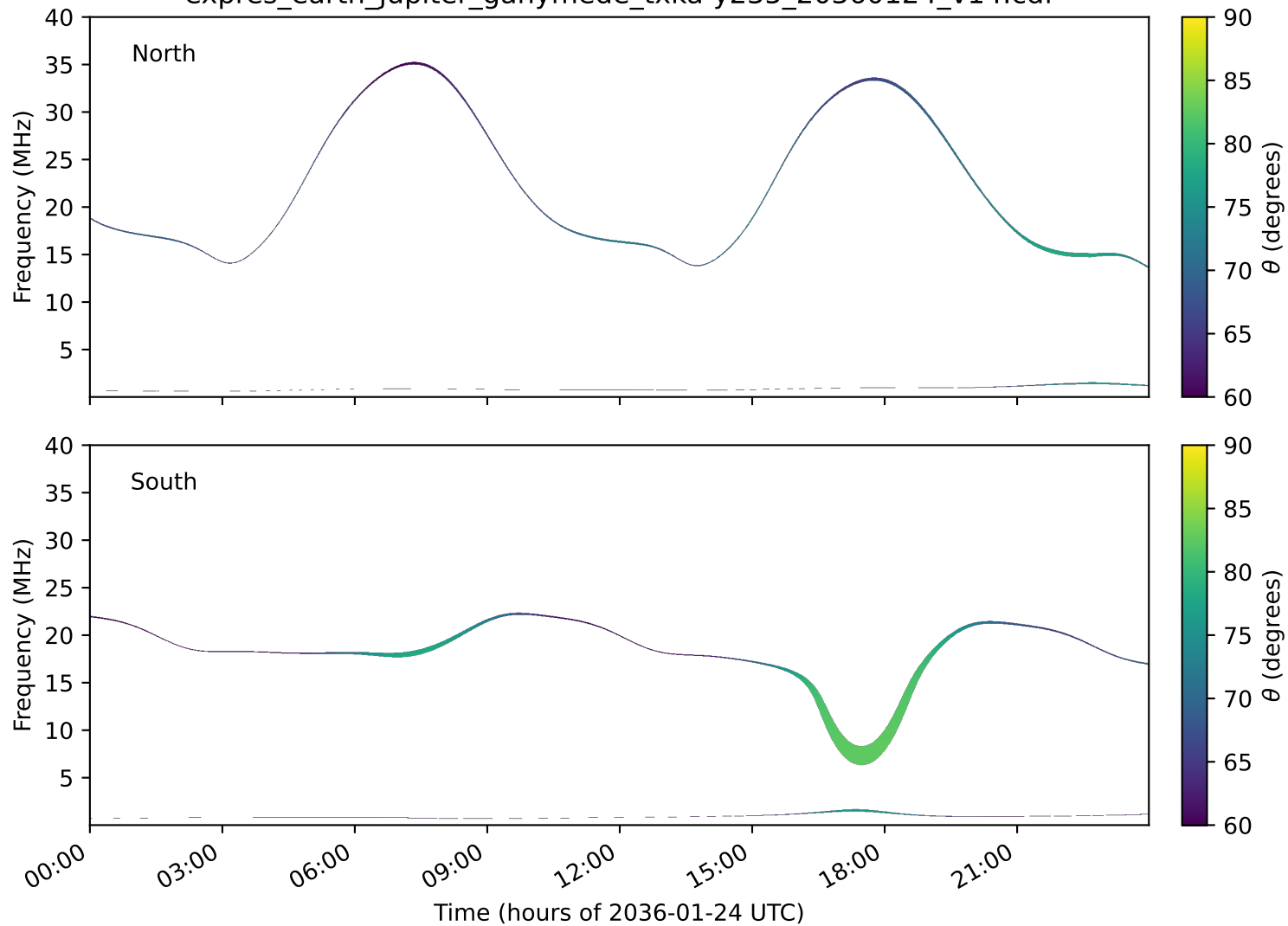
expres_earth_jupiter_ganymede_txka-y235_20360124_v14.cdf
