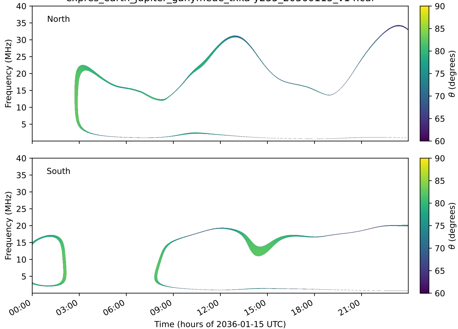
expres_earth_jupiter_ganymede_txka-y235_20360115_v14.cdf
