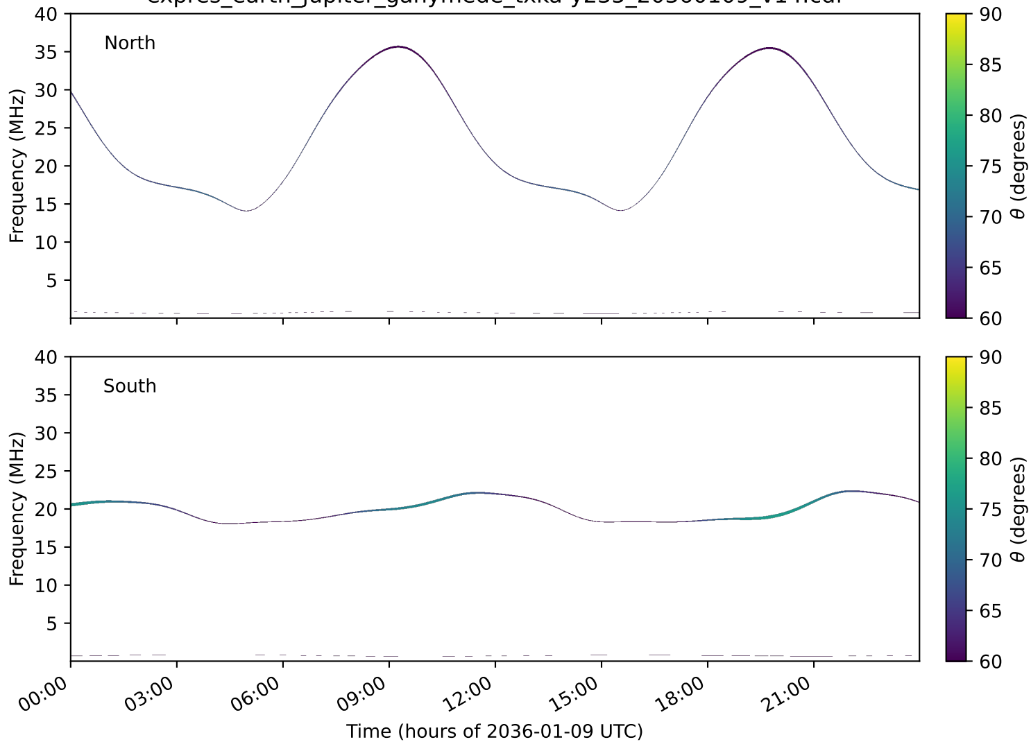
expres_earth_jupiter_ganymede_txka-y235_20360109_v14.cdf
