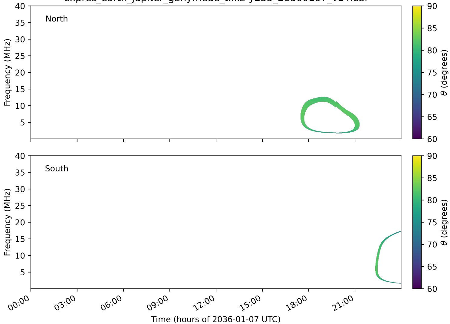
expres_earth_jupiter_ganymede_txka-y235_20360107_v14.cdf
