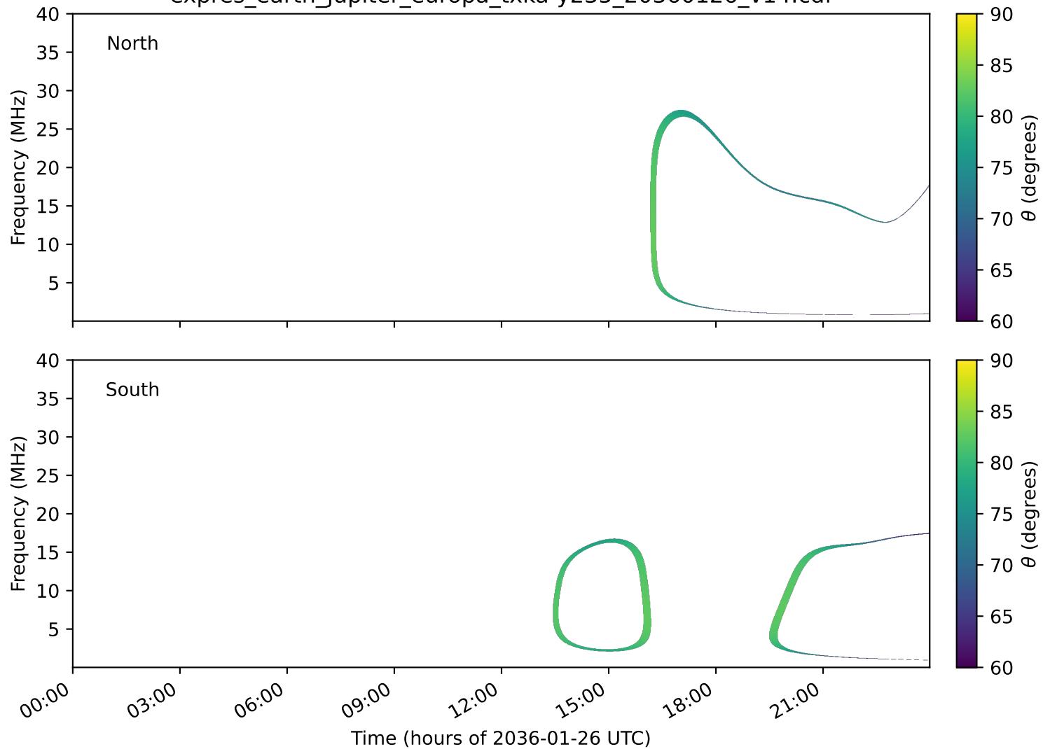
expres_earth_jupiter_europa_txka-y235_20360126_v14.cdf
